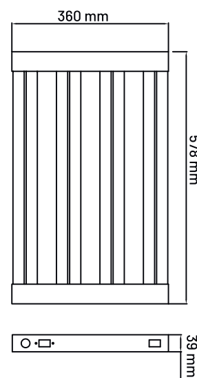
PC Cover
